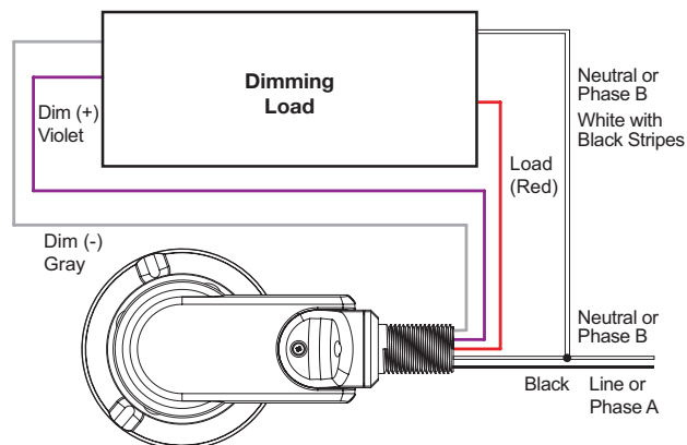
FSP-2x1-B wiring with dimming ballast or LED driver
