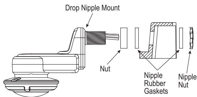
Figure 3. Installing the FSP-2x1B-D to a pole using the optional spacer
