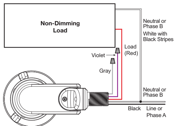
FSP-2x1-B wiring with non-dimming load
