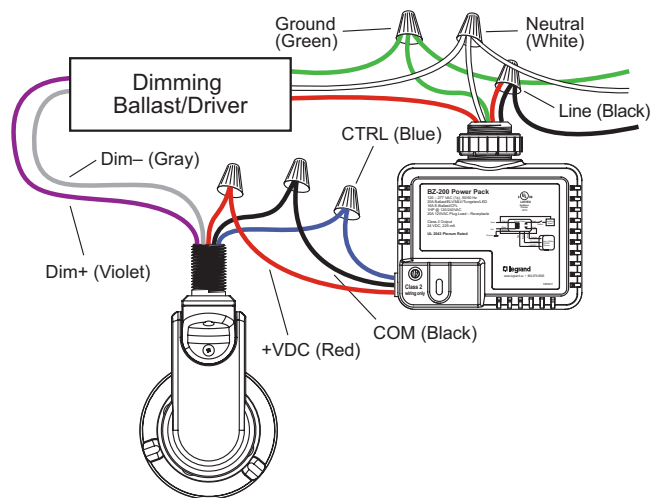
FSP-201B wiring with dimming ballast or LED driver and power pack for on/off control. If using a non-dimming ballast/driver, simply cap the gray and violet leads
