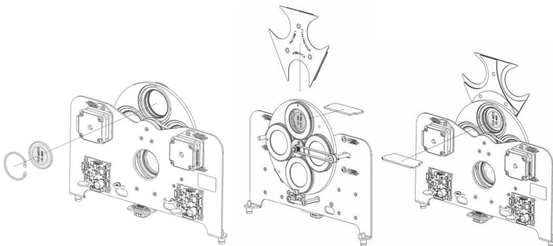
Change Image kit (4 Gobo) DIVUM 50K with App
