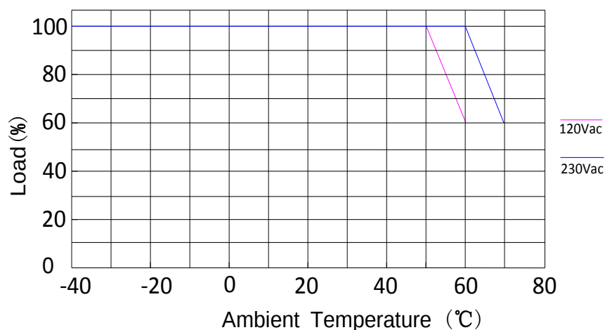
Derating Curve
