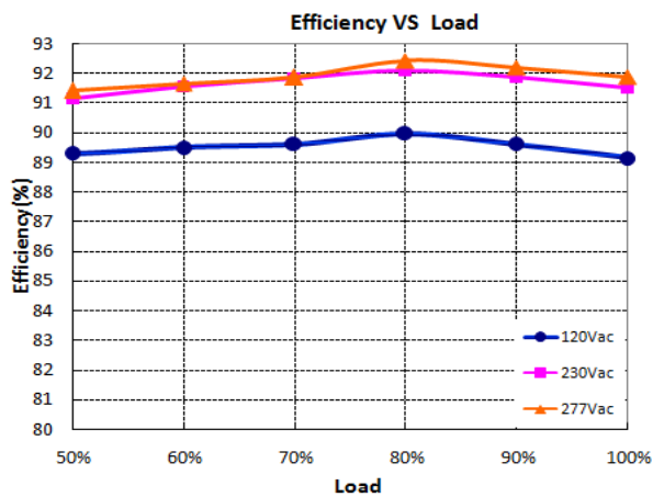
X6-105Y150 (Io=0.70A)
