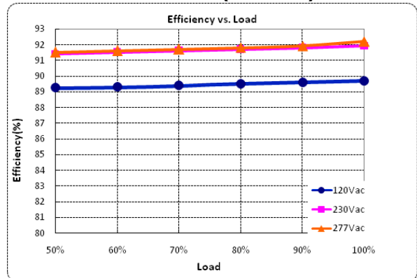
X6-105Y062 (Io=2.50A)
